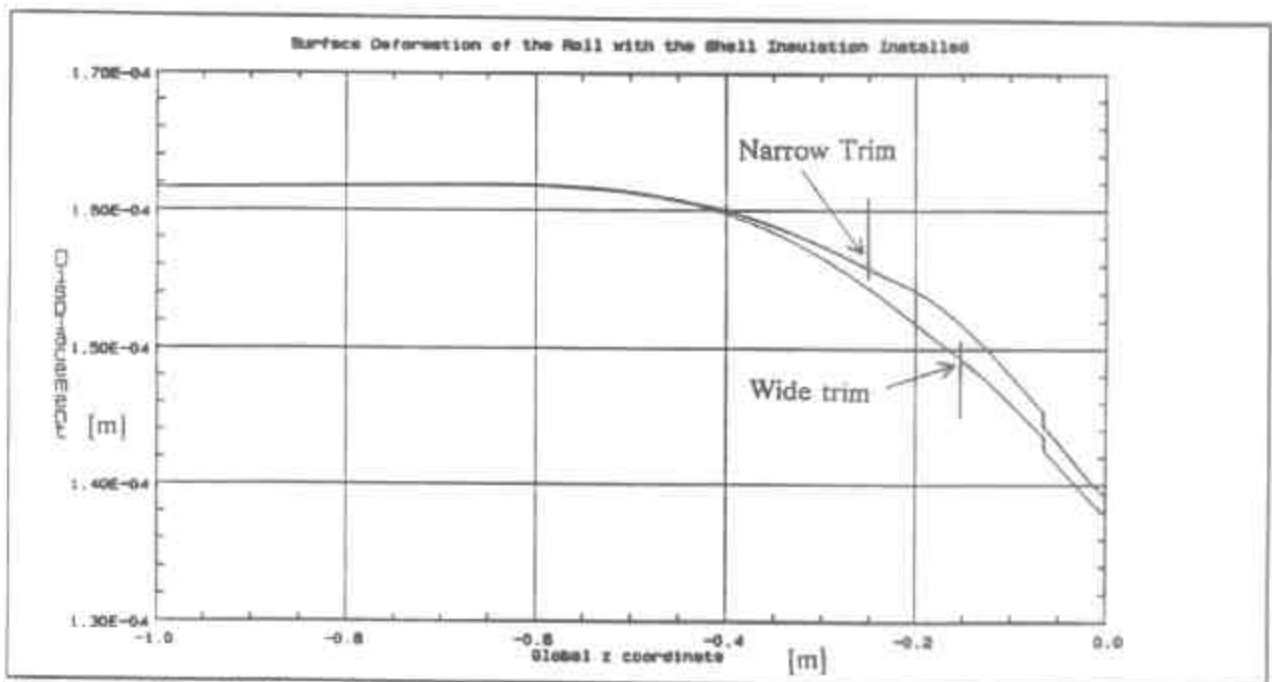
Figure 8 The shell surface deformation for the insulated shell with wide and narrow trim.
