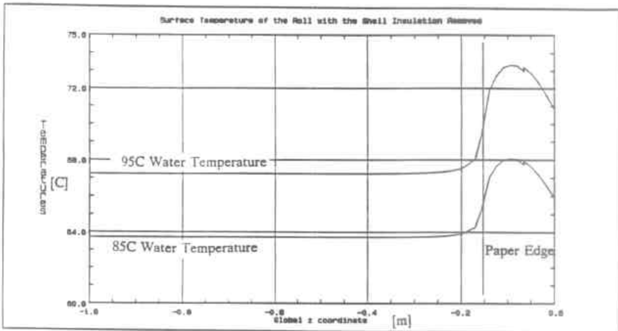
Figure 9 Surface temperature of the roll with insulation removed at two different setpoint temperatures.
