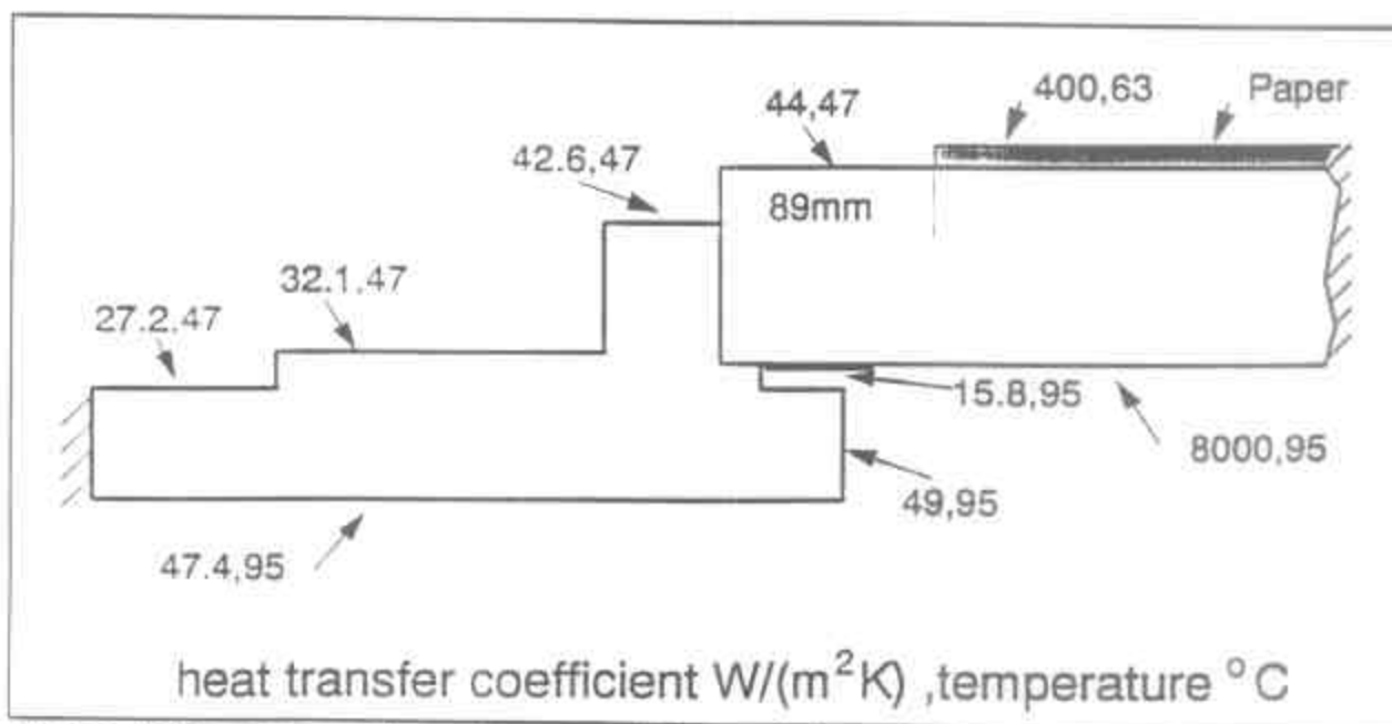
Figure 5 The thermal boundary conditions of the calender stack.
