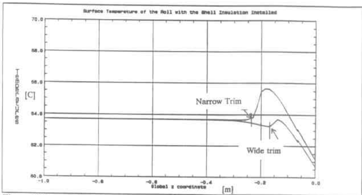
Figure 7 The surface temperature profile of the insulated calender shell with wide and narrow trim.
